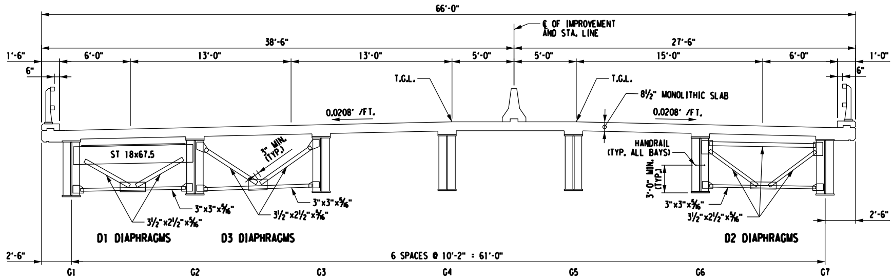
TRANSVERSE SECTION SCALE: \frac{1}{8}" = 1'-0"
