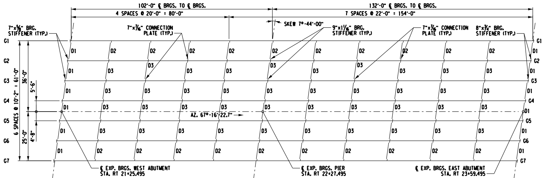
FRAMING PLAN
