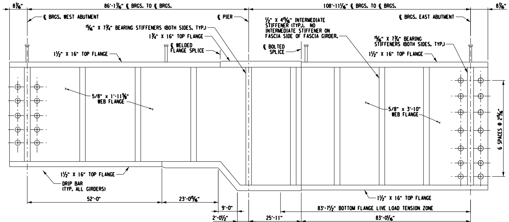
GIRDER ELEVATION
