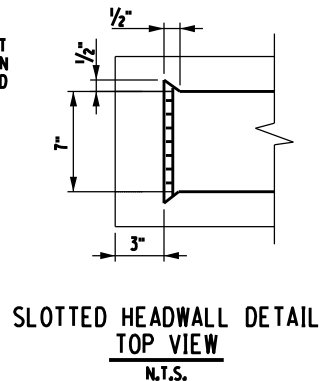
DETAIL B PRECAST CONCRETE OUTLET HEADWALL 6 INCH LATERAL OUTLET PIPES ITEM 605.21015025 N.T.S.
