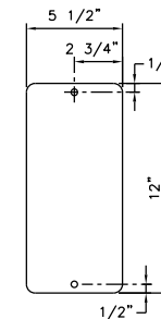
SINGLE DELINEATOR (WHITE OR YELLOW) N.T.S.
