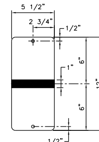
DOUBLE DELINEATOR (WHITE OR YELLOW) N.T.S.
