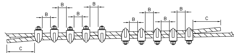
WIRE ROPE DETAIL BB WIRE ROPE SPLICING N.T.S.
