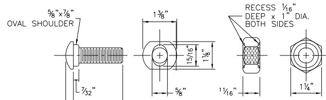
2" RAIL BLOCKOUT BOLT/NUT SCALE: 6" = 1'-0"
