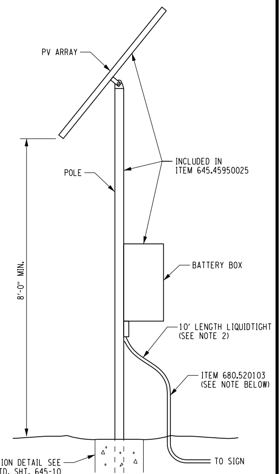
ELEVATION SOLAR POWER STATION ITEM 645.45950025 (WHERE APPLICABLE) N.T.S.
