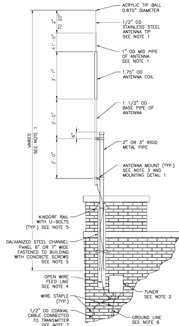
BUILDING MOUNT (NTS)
