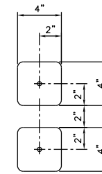
DOUBLE SNOWPLOW MARKER (GREEN) N.T.S.
