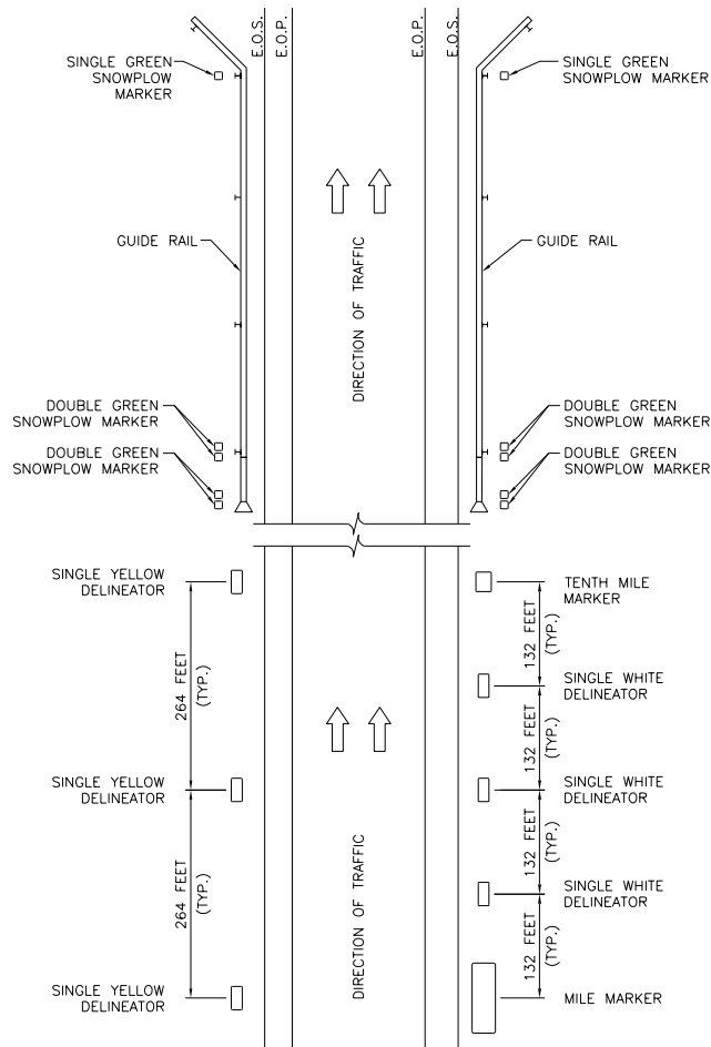
MARKER AND DELINEATOR LAYOUT FOR THRUWAY MAINLINE
