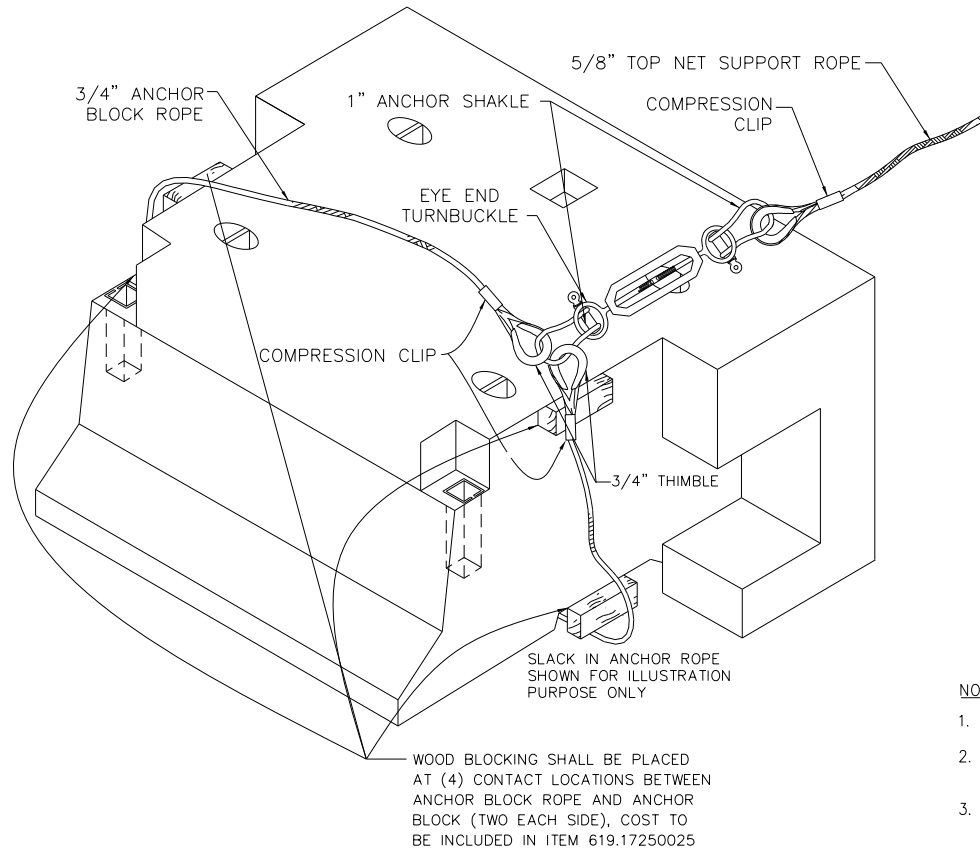
COLUMN SUPPORT ANCHOR BLOCK DETAIL "A" NTS
