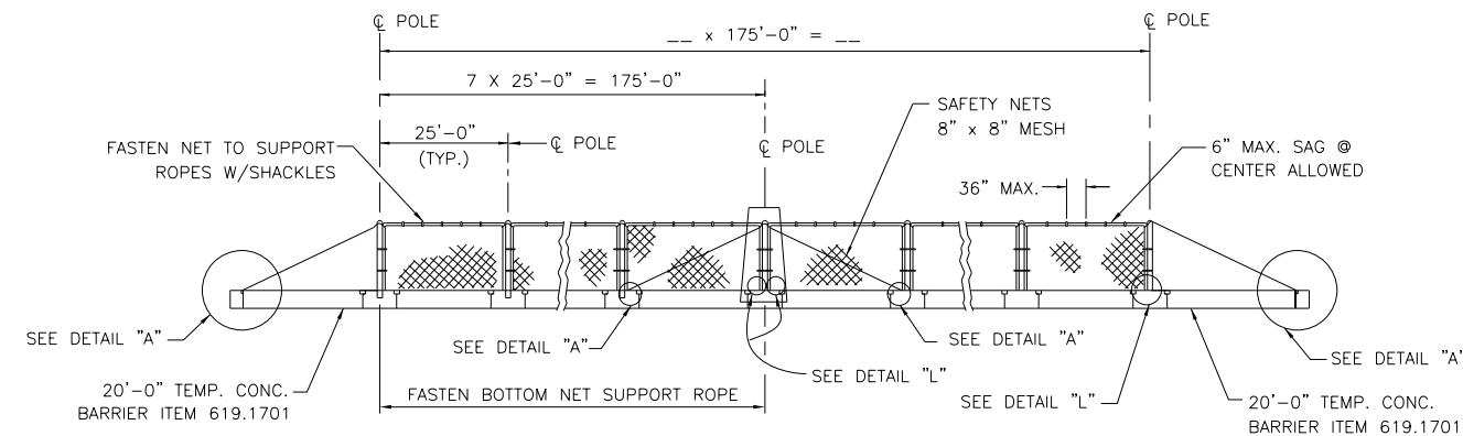
ELEVATION VIEW
