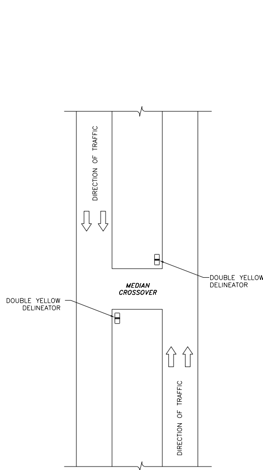
DELINEATOR LAYOUT MEDIAN CROSSEOVERS
