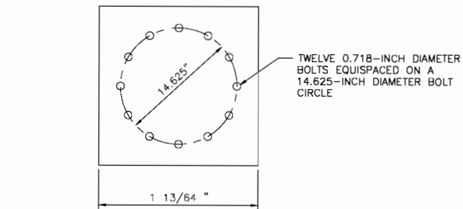
CONNECTION OF ANTENNA BASE TO MOUNTING PLATE ON TOP OF STEEL TOWER (NTS)
