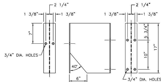
END VIEW ELEVATION END VIEW
