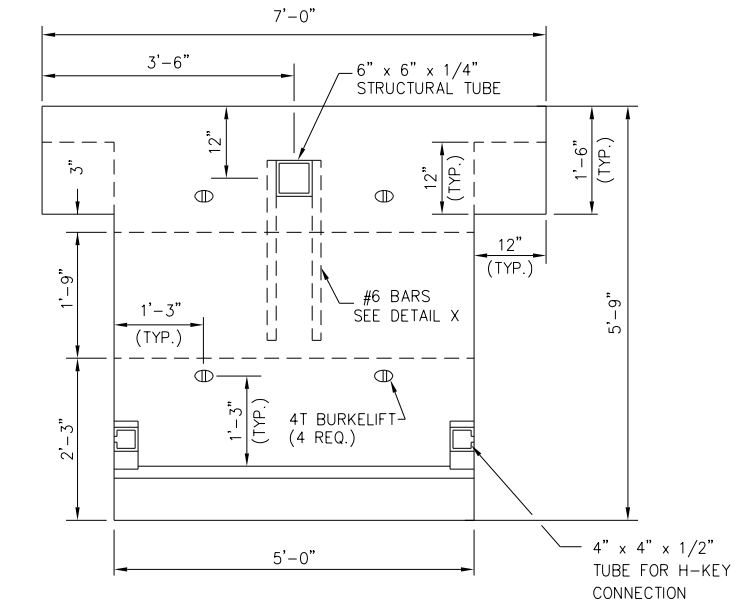
COLUMN SUPPORT PLAN VIEW N.T.S.
